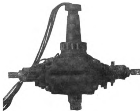
HUB MOTOR, SHOWING STUB JOURNAL AND WIRES, ROLLER BEARING AND DRIVE EQUALIZER.
